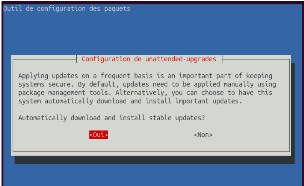
Figure 13 unattended-upgrades
